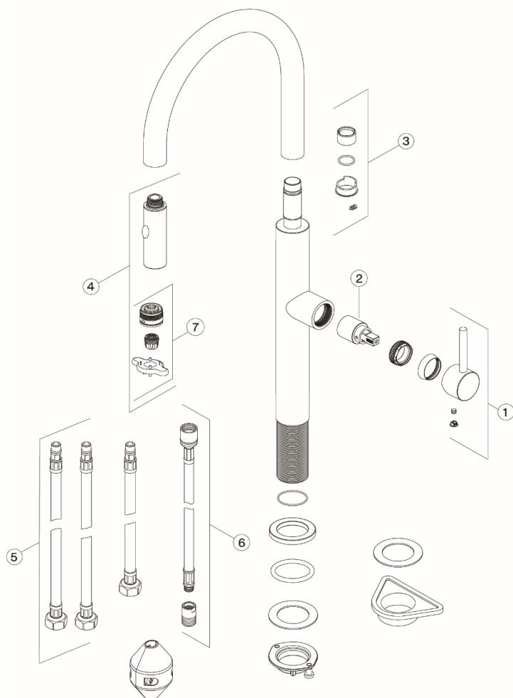
Tap Pescara J Pull Down Spray HP IBK 115.0741.695
